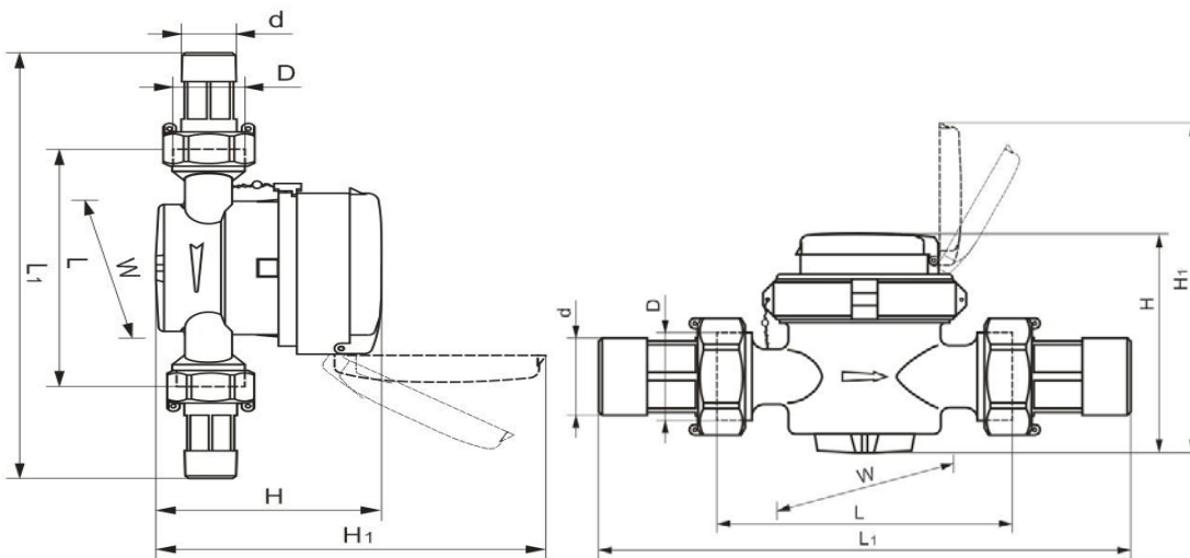
INSTALACION VERTICAL
